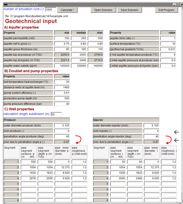
Figure 5. DoubletCalc input screen showing well inclination and automatically calculated penetration angle skin. Additionally, a 'skin producer' and / or 'skin injector' can be specified.
